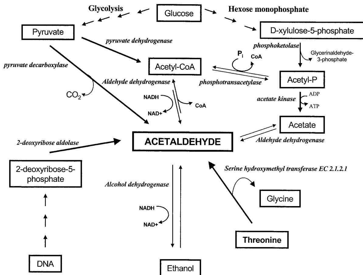
FIG. 1. Overview of the different metabolic pathways in LAB that could lead to acetaldehyde formation. Acetyl-CoA, acetyl coenzyme A.
