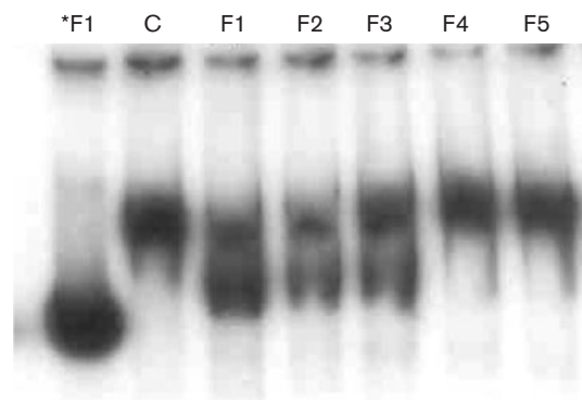
Fig. 5. Electrophoretic mobility shift assay: competition. *F1, radiolabelled fragment P_{metC}F1-P_{metC}R ; C, P_{metC} -CmbR complex; F1, F2, F3, F4 and F5, unlabelled deletion variants.
