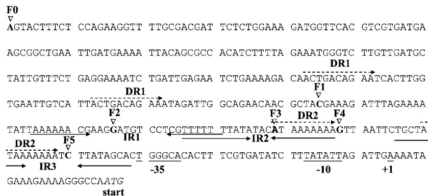
Fig. 1. Complete nucleotide sequence of P_{\text{metC}} (F0). F1, F2, F3, F4 and F5 represent the truncated fragments. The first nucleotide in each truncated fragment is boldface and indicated by a downward pointing arrowhead. Inverted repeats (IR1, IR2 and IR3) and direct repeats (DR1 and DR2) are represented by solid and dashed arrows, respectively. The -35 and -10 sequences, transcription start (+1) and start codon are indicated.
