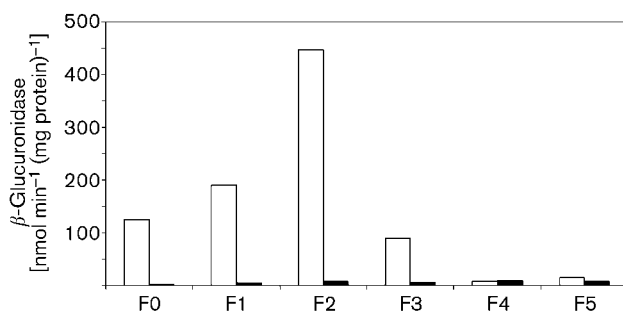
Fig. 2. \beta -Glucuronidase activities of promoter- gusA fusions with F0, F1, F2, F3, F4 and F5 promoter fragments of P_{metC} . White bars, CDM containing 0.1 \times Met; black bars, CDM containing 10 \times Met/ 10 \times Cys. Results are the means of three independent experiments.
